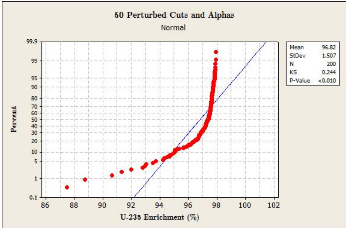
Figure 13. K-S Test for 50 Perturbed Cuts and Alphas
