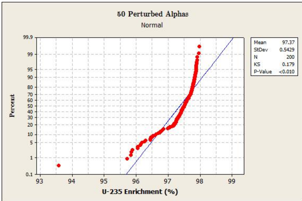
Figure 11. K-S Test for 50 Perturbed Alphas
