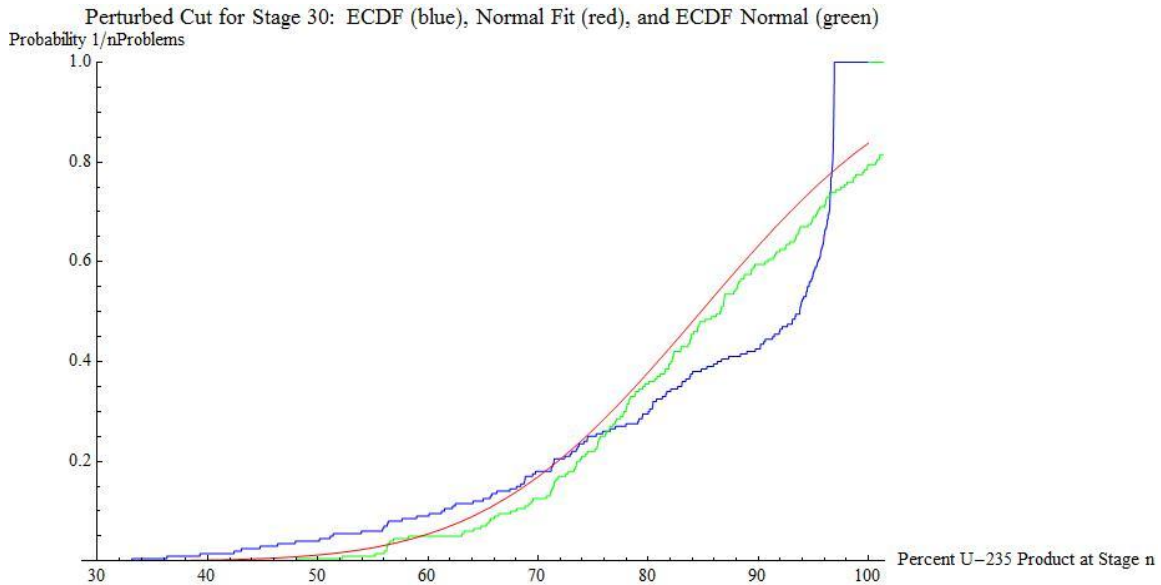
Figure 30. Perturbed Cut at Stage 30
