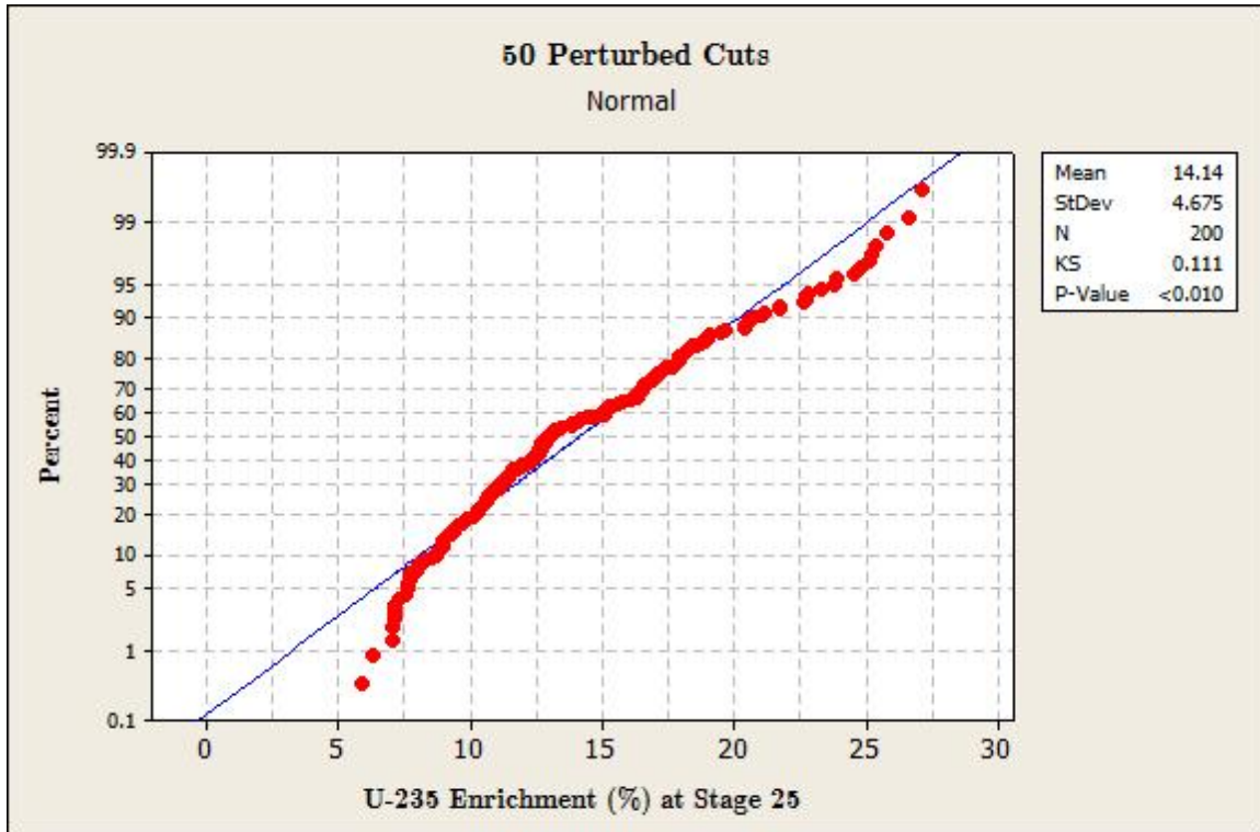
Figure 9. K-S Test for 50 Perturbed Cuts, ^{235}\text{U} at Stage 25
