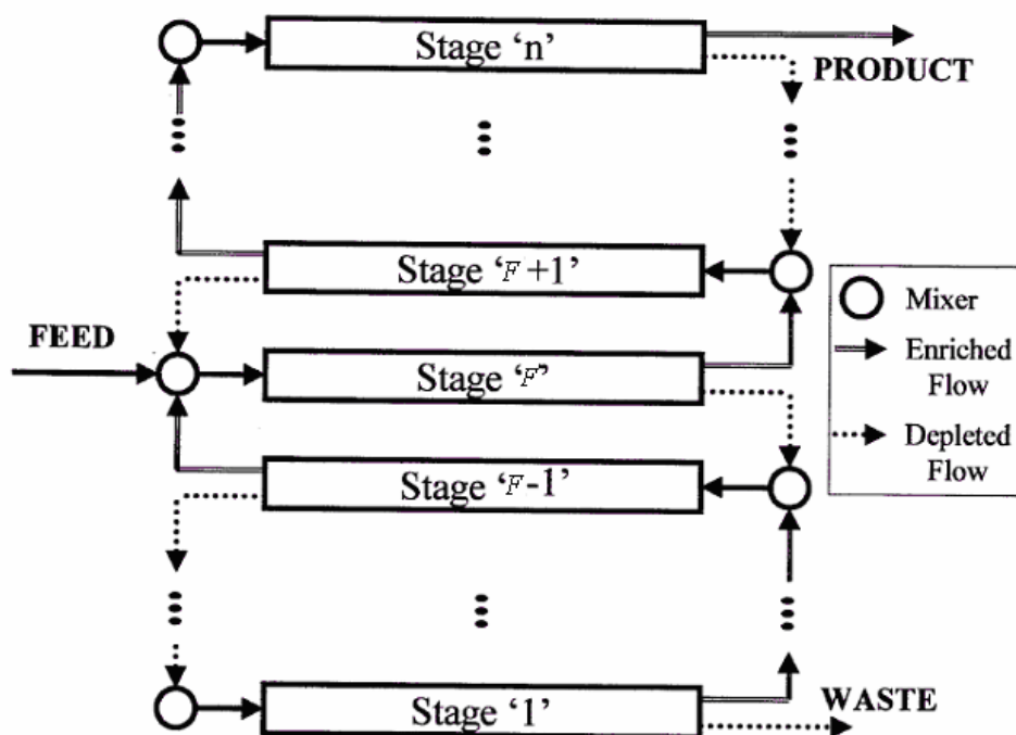
Figure 1. Example of 1 up-1 down Cascade
