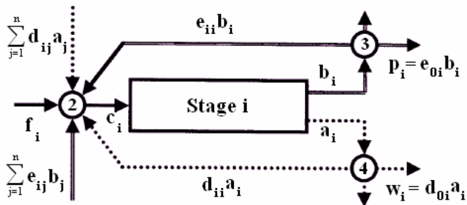
Figure 2. Possible Flow Paths for Stage i
