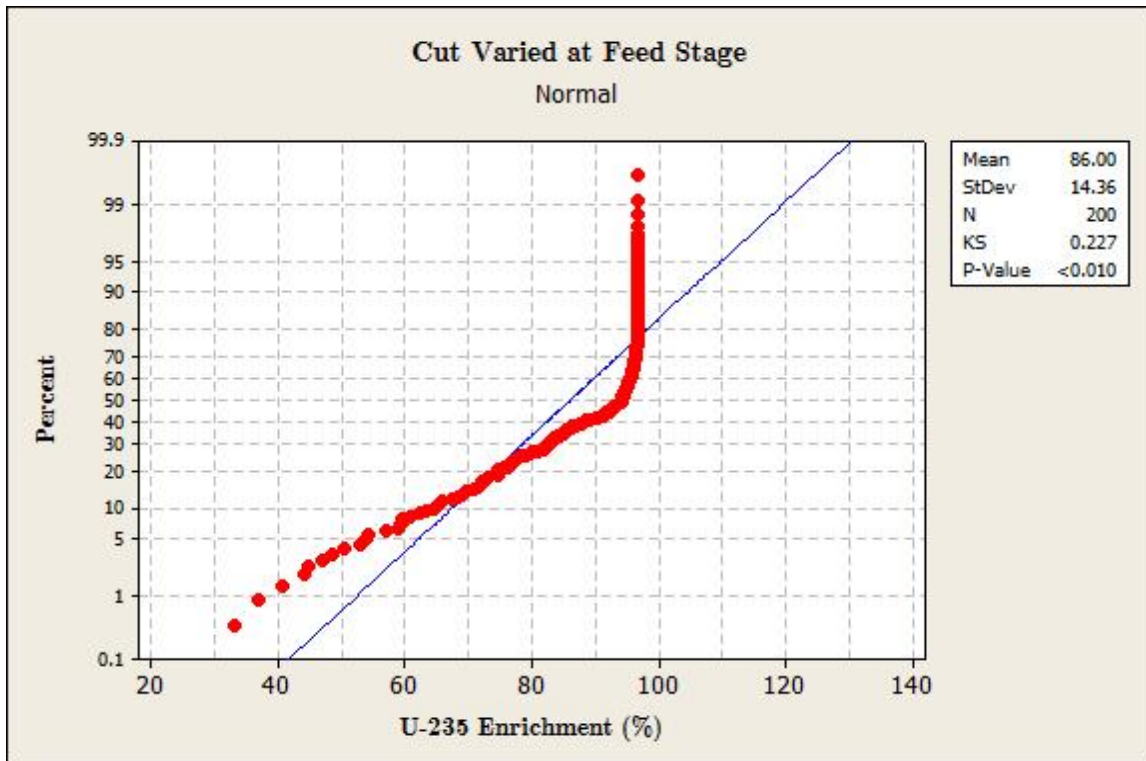
Figure 25. K-S Test for Varying Cut at Feed Stage
