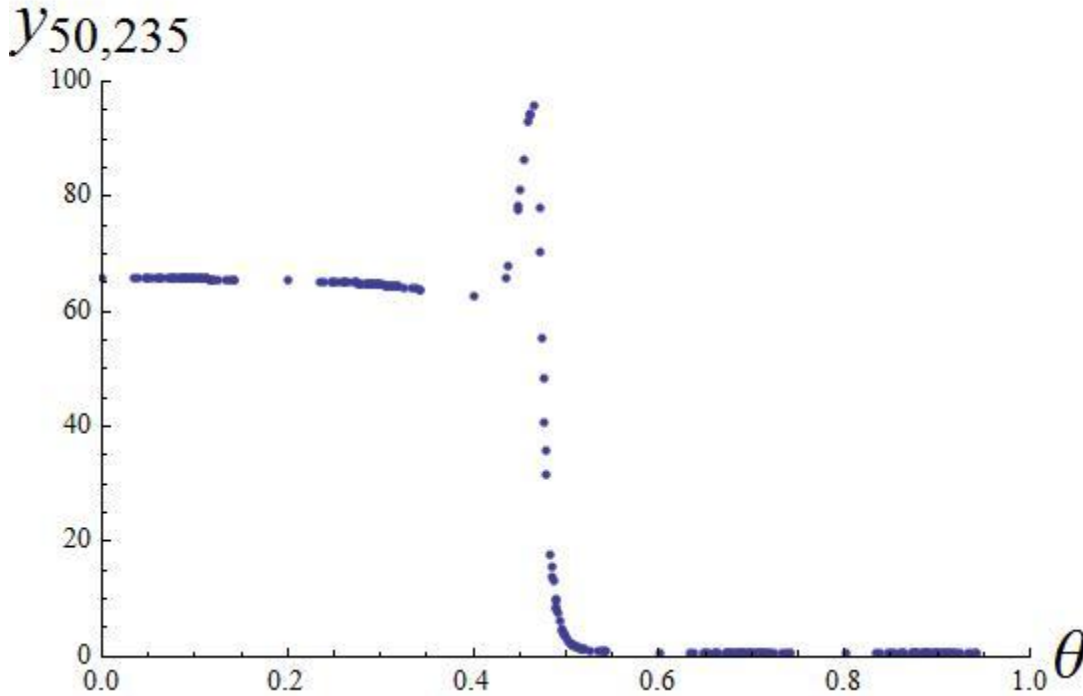
Figure 14. ^{235}\text{U} Product as a Function of Cut
