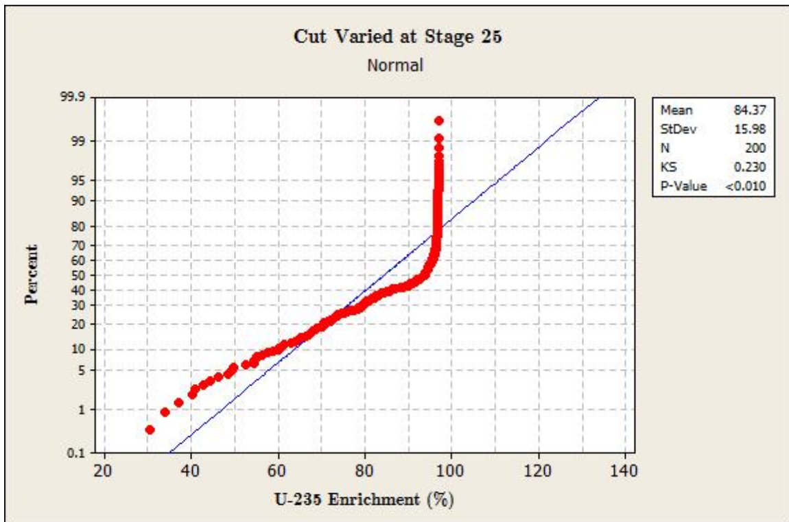
Figure 19. K-S Test for Varying Cut at Stage 25
