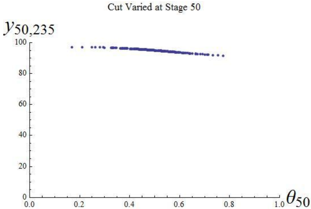
Figure 23. Enriched ^{235}\text{U} Product as a Function of Cut for Stage 50
