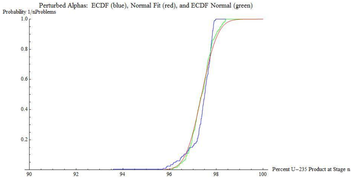
Figure 10. Perturbed Alphas for all Stages
