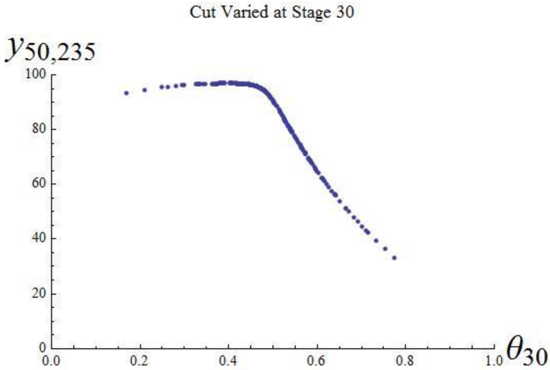
Figure 32. Enriched ^{235}\text{U} Product as a Function of Cut for Stage 30
