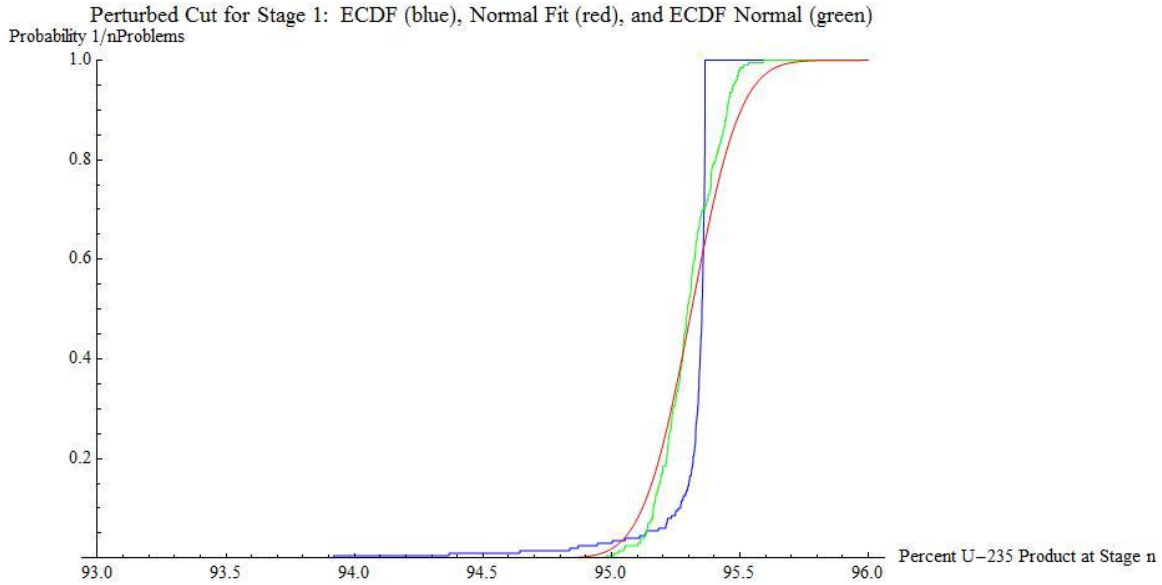
Figure 15. Perturbed Cut at Stage 1
