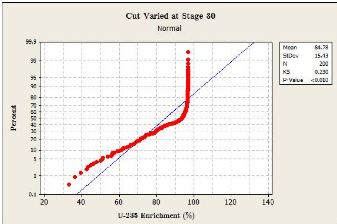
Figure 31. K-S Test for Varying Cut at Stage 30
