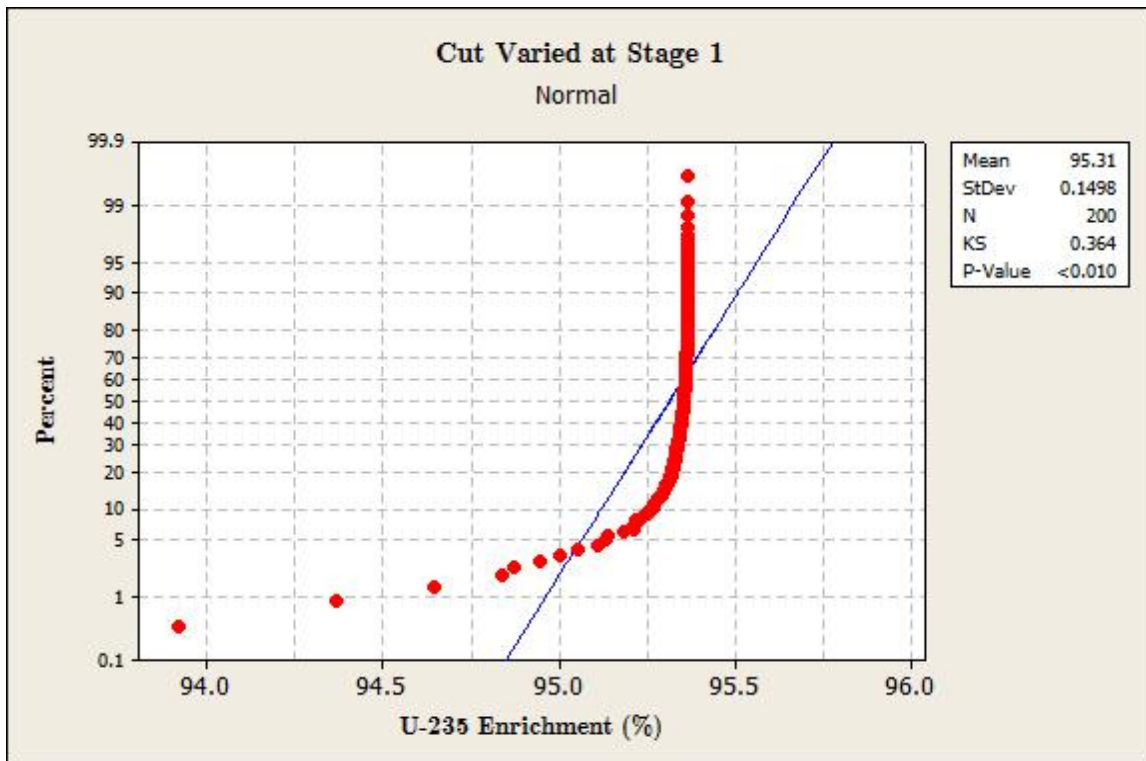
Figure 16. K-S Test for Varying Cut at Stage 1
