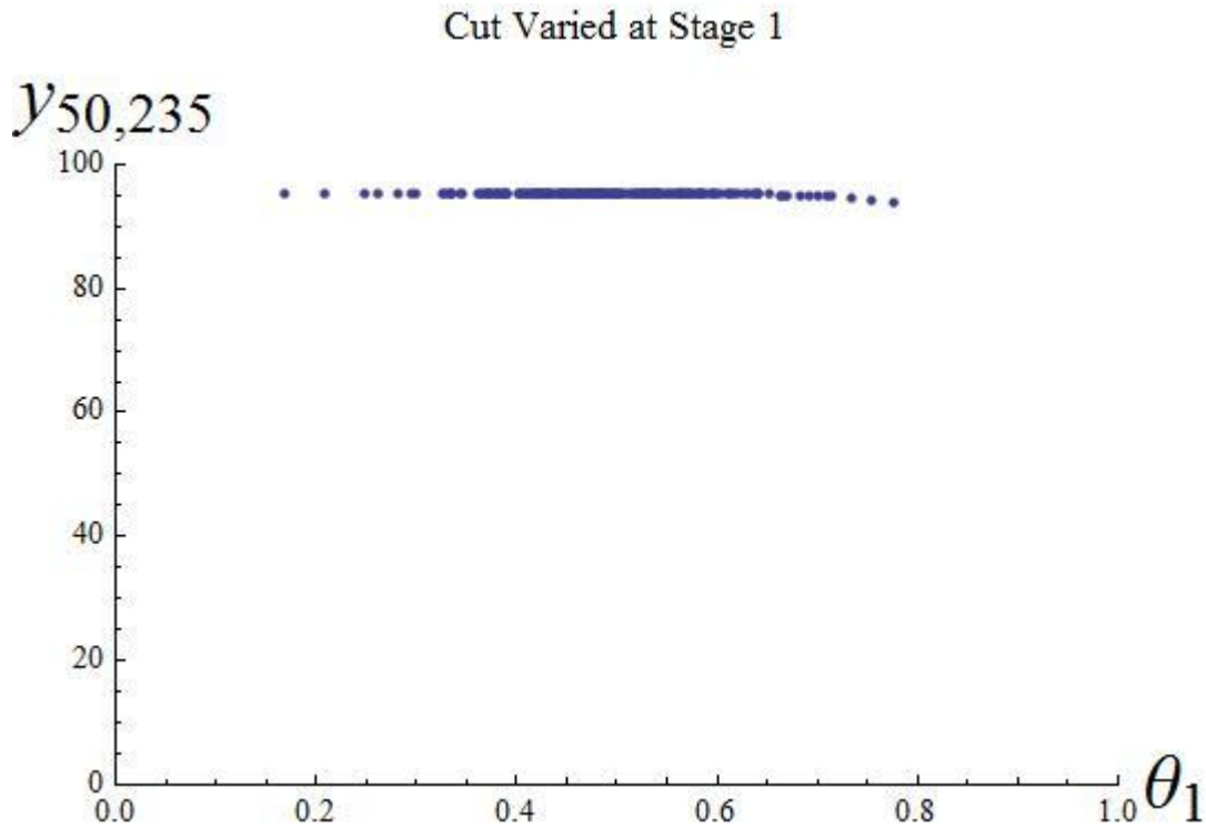
Figure 17. Enriched ^{235}\text{U} Product as a Function of Cut for Stage 1
