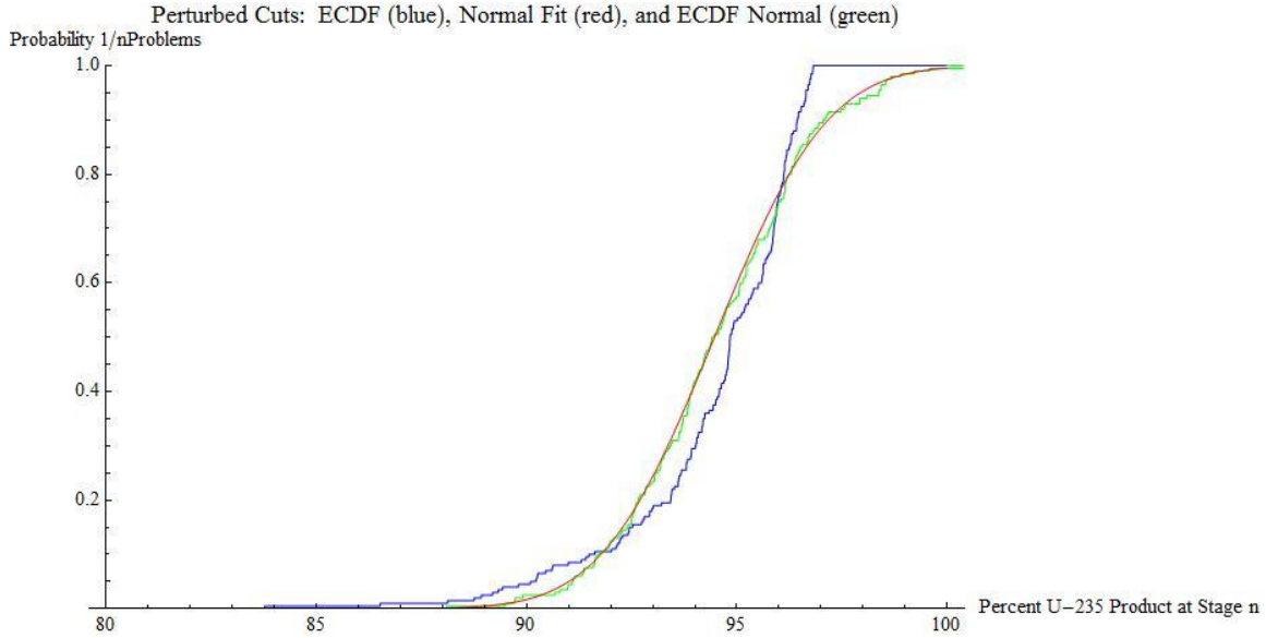
Figure 6. Perturbed Cuts for all Stages, ^{235}\text{U} at Stage 50
