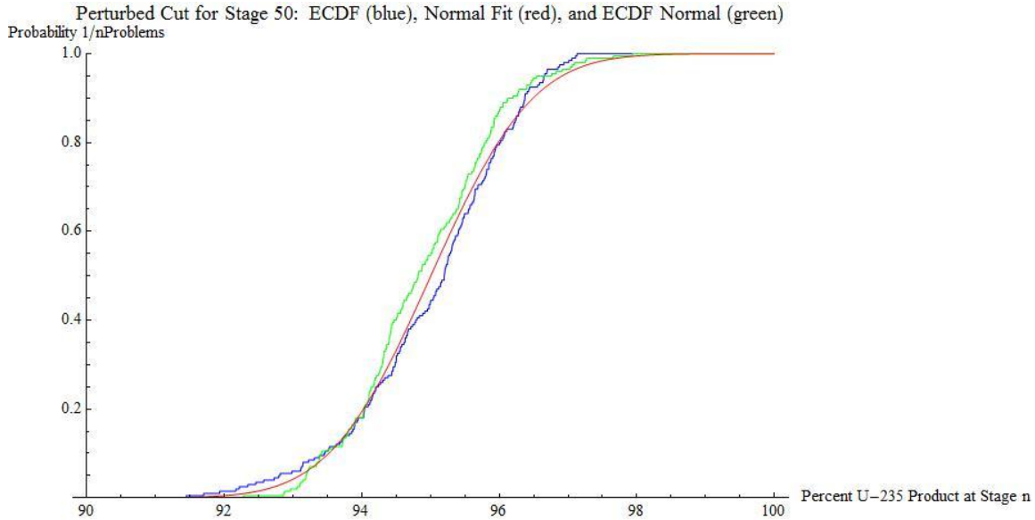
Figure 21. Perturbed Cut at Stage 50
