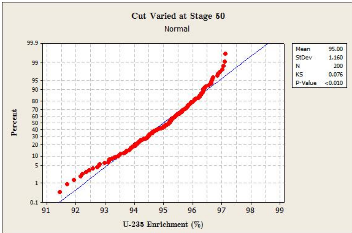
Figure 22. K-S Test for Varying Cut at Stage 50
