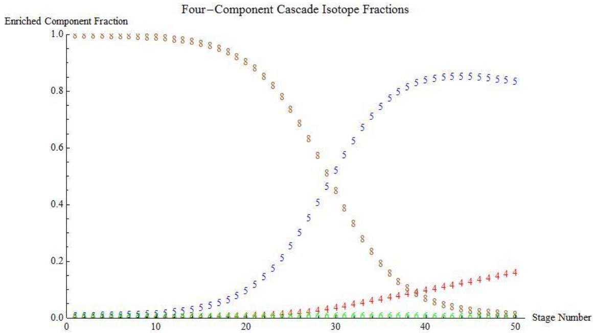
Figure 5. U Component Fractions at Each Stage
