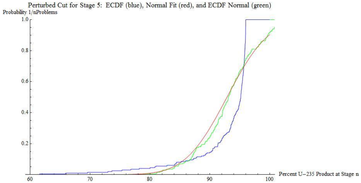
Figure 27. Perturbed Cut at Stage 5
