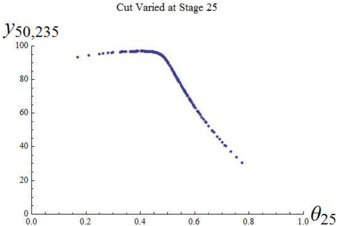
Figure 20. Enriched ^{235}\text{U} Product as a Function of Cut for Stage 25
