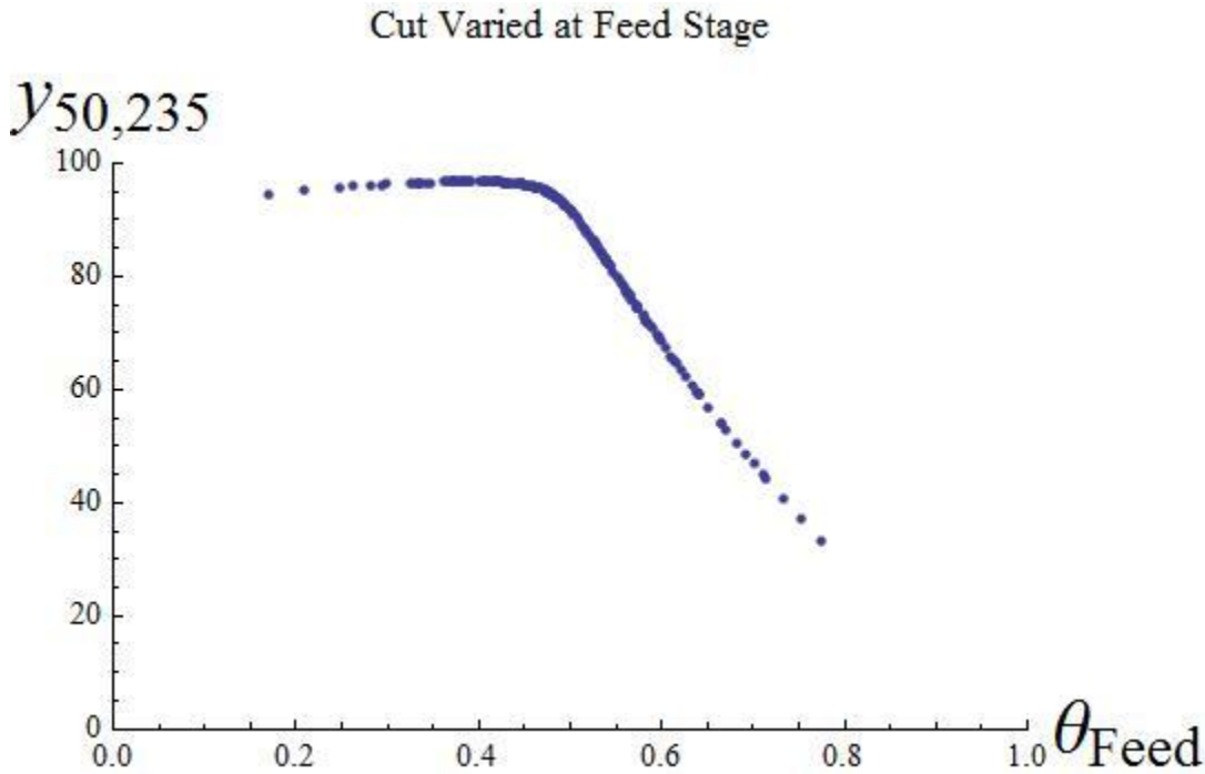
Figure 26. Enriched ^{235}\text{U} Product as a Function of Cut for Feed Stage
