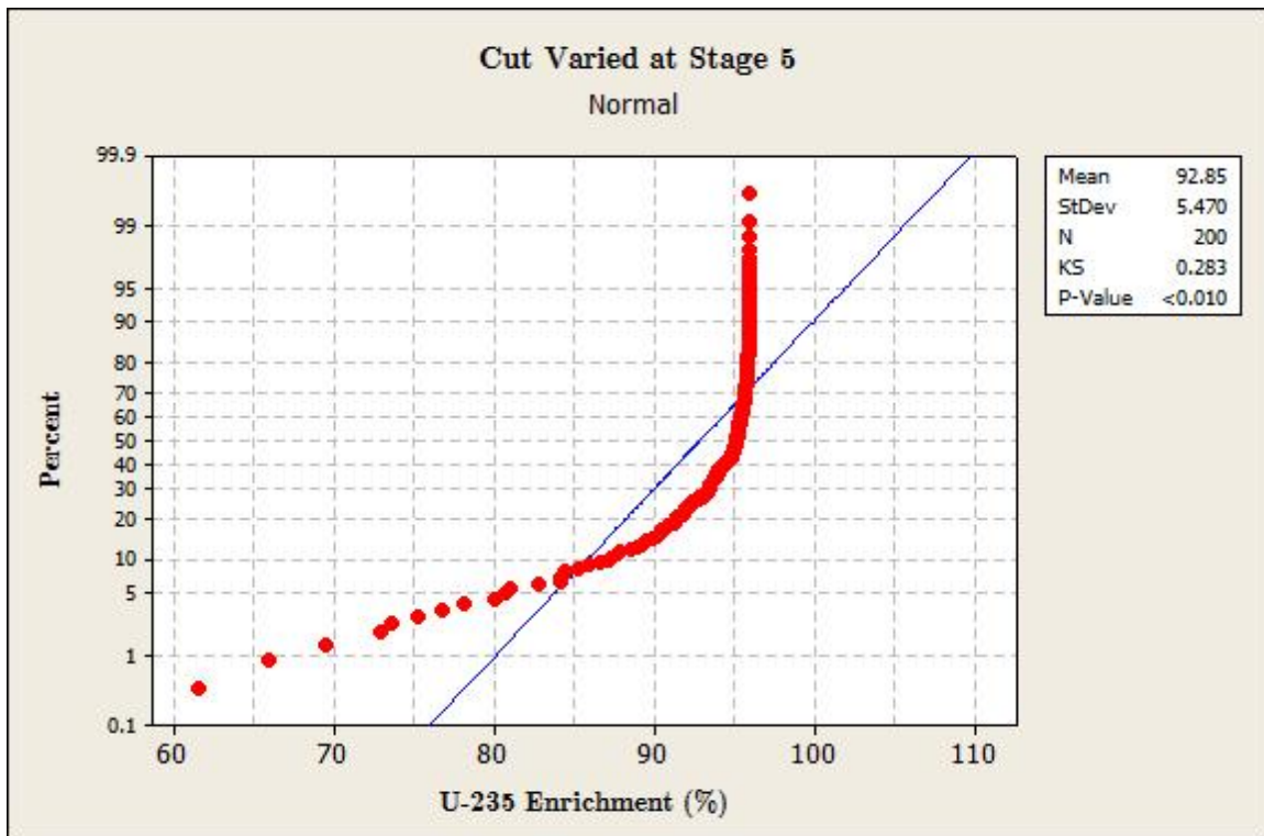
Figure 28. K-S Test for Varying Cut at Stage 5
