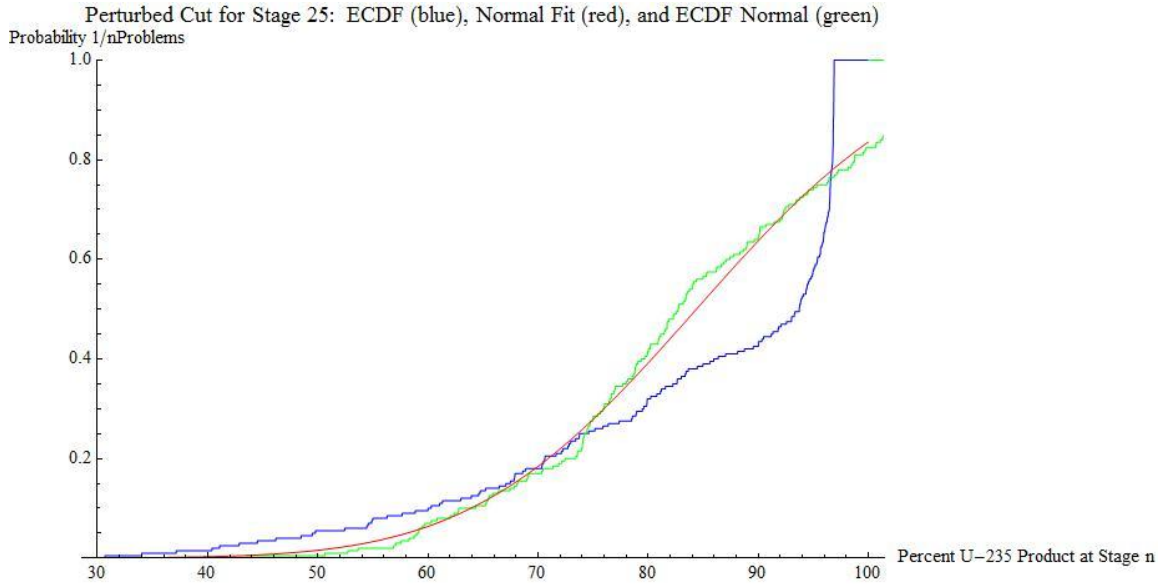
Figure 18. Perturbed Cut at Stage 25
