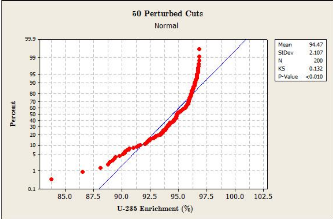
Figure 7. K-S Test for 50 Perturbed Cuts, 235 U at Stage 50
