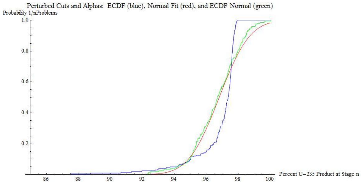
Figure 12. Perturbed Cuts and Alphas for all Stages
