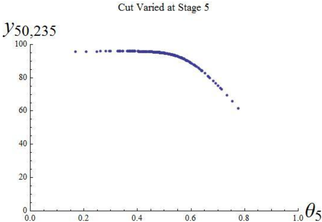
Figure 29. Enriched ^{235}\text{U} Product as a Function of Cut for Stage 5
